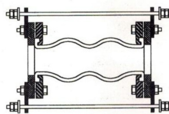
WITH CONTROL RODS
